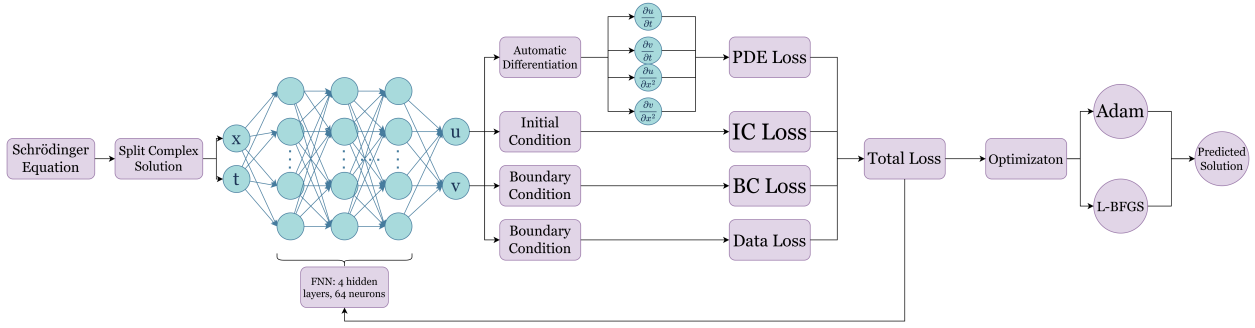
Figure 3: Diagram of solveing Schrödinger with PINN
